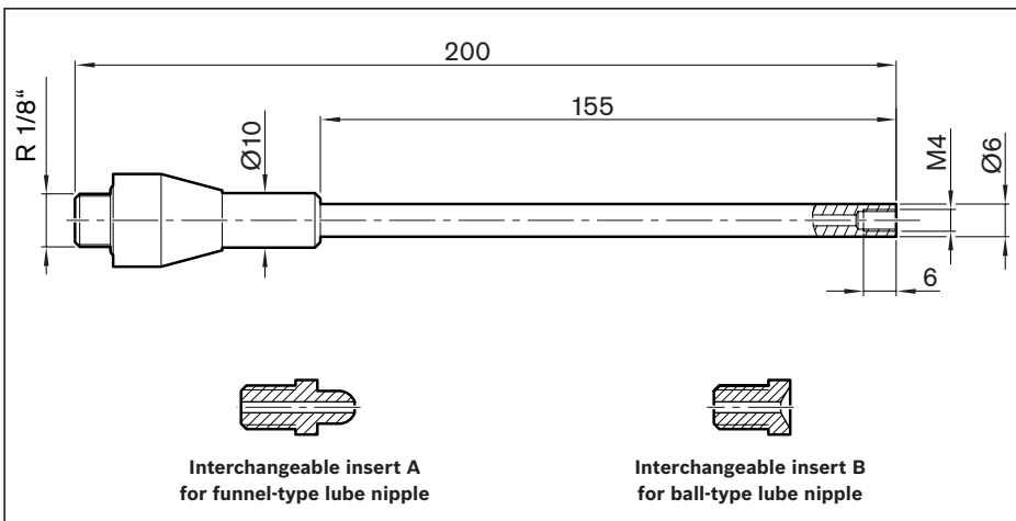
Nozzle pipe
